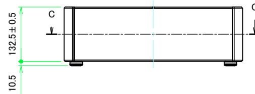
B-B (1:6.5)
